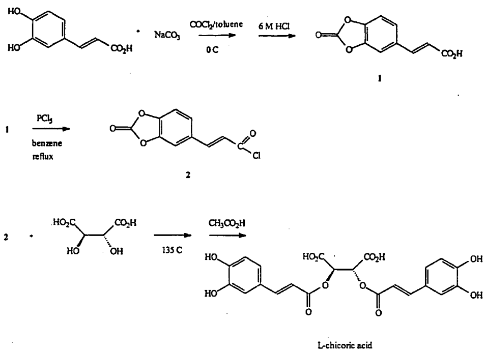
Scheme 1 Synthesis of L-chicoric acid
